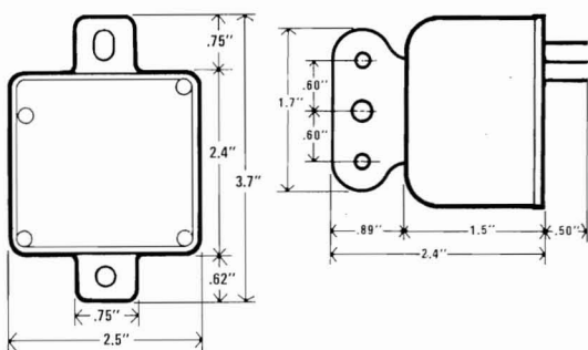
PLASTIC CASE
