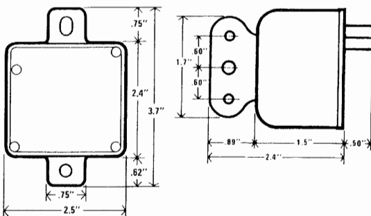
PLASTIC CASE
